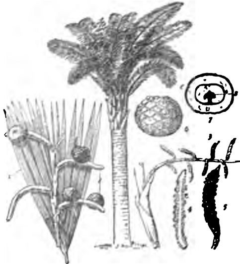
FIG 6.—Sago Palm ( Metroxylon Sagus ).
