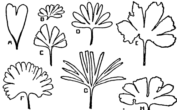
FIG. 18.—Leaves of Ginkgoales .
