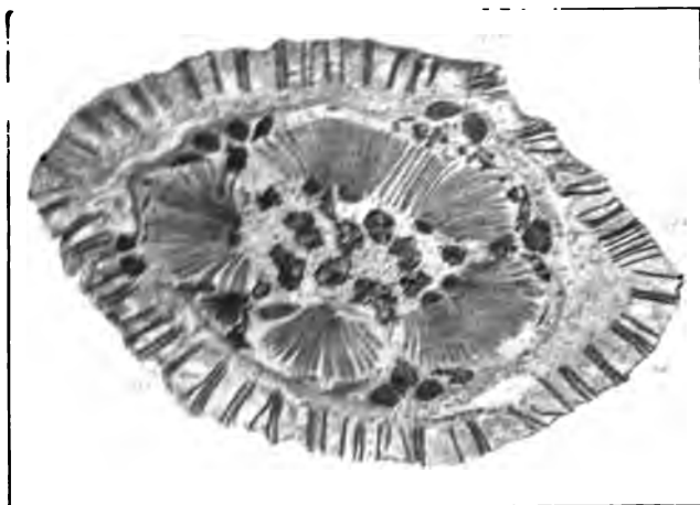
Fig. 21. Lycopodium oldhamium . Transverse section of stem, showing the pith containing groups of sclerotic cells, the primary xylem strands, secondary wood and phloem, pericycle and cortex. l 1 l 5 , leaf traces, numbered according to the phyllotaxis, l 5 belonging to the lowest leaf of the five; ph , a group of primary phloem; pd , periderm, formed from pericycle.
