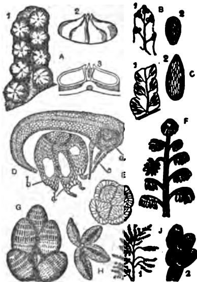
FIG. 15.—Group of Palaeozoic fructifications of Ferns or
