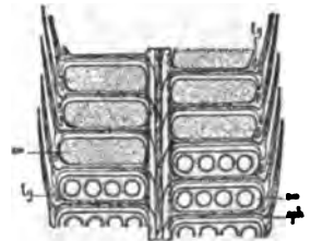
FIG. 10.— Lepidostrobus . Diagram of cone, in longitudinal section. ax, Axis, bearing the sporophylls (sph) on each of which a sporangium (sw) is seated. lg, Ligule.
