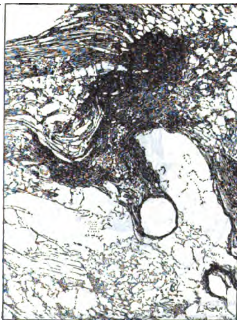
FIG. 24.—Capitate gland on the cupule of Lagenostoma Lomaxii . (X 70.)
