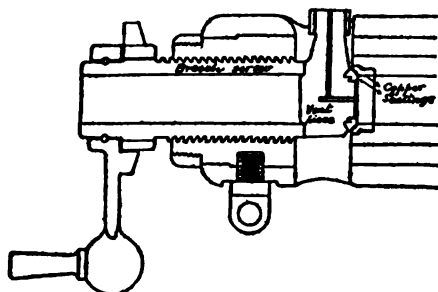
FIG. 10.—Armstrong B.L. Arrangement.
