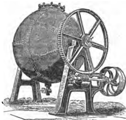
FIG. 1.—Revolving Spherical Rag Boiler.
