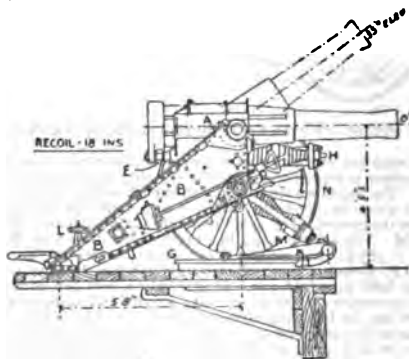
FIG. 72.—Diagram of British 6-in. B.L. Howitzer.
