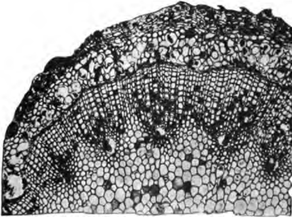
Fig. 1.— Calamites . Part of transverse section of a young stem, showing pith, vascular bundles with secondary wood, and cortex. From a photograph (Scott, "Studies").
