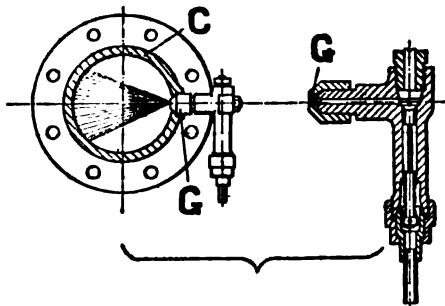
FIG. 15.—Crossley Oil Engine.
