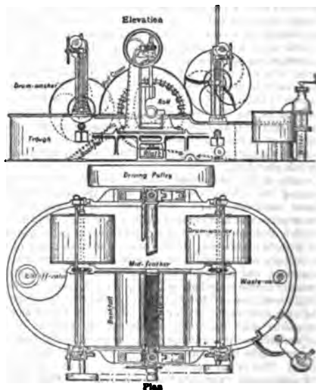
FIG. 2.—Rag-breaking Engine.
