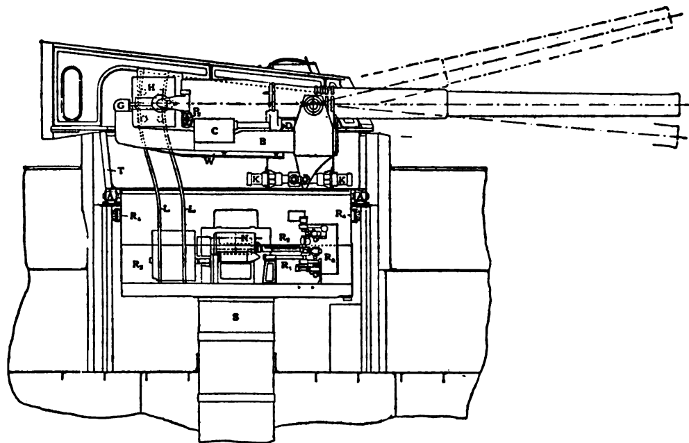
FIG. 91.—Diagram of 12-in. Gun Mounting, "Dreadnought" type.
