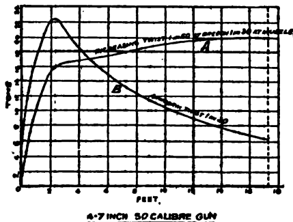
FIG. 31.—Pressure Curves (uniform and increasing twist).
