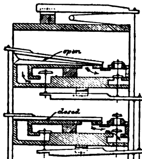
FIG. 13.—Pneumatic Lever.
