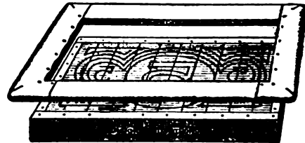
FIG. 11.—Mould and Deckel for hand-made paper.
