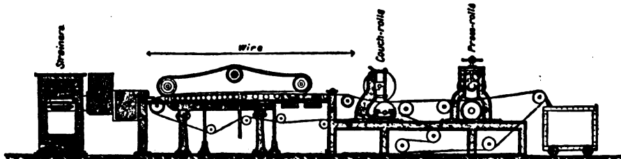
FIG. 4.—"Press-Pâte," or Half-stuff Machine.
