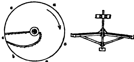
FIG. 10.—Convex Revolving Slime-table.
