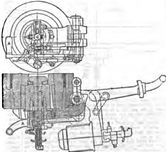
FIG. 43.—Breech Mechanism, Modern 6-in. Gun.
