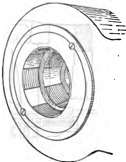
FIG. 39.—Elswick Coned Screw.
