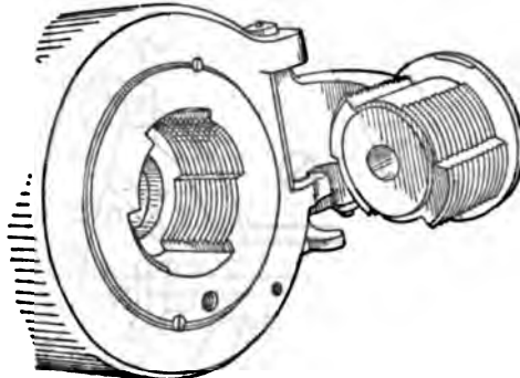
FIG. 38.—Welin Breech Screw.
