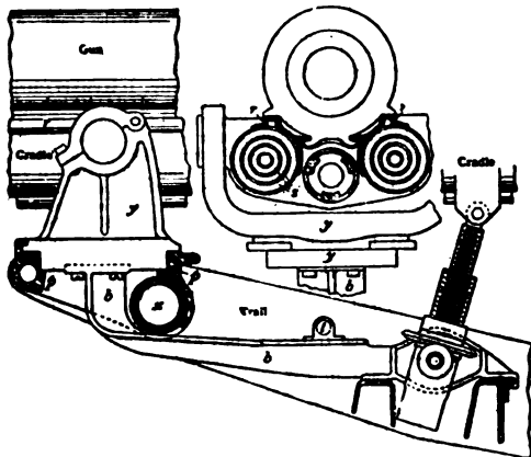
FIG. 71.—Diagram of 4.7-in. Siege Gun, U.S.A.
