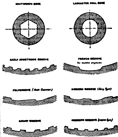
FIG. 22.—Sections of Rifling.
