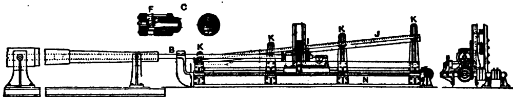
FIG. 21.—Rifling Machine.
