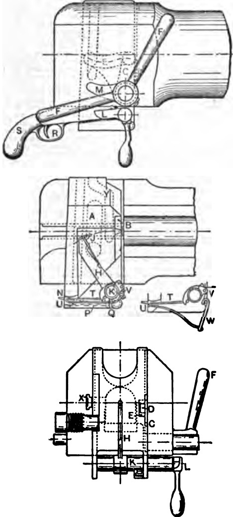
FIG. 34.—Hotchkiss Q.F. Breech Mechanism.
