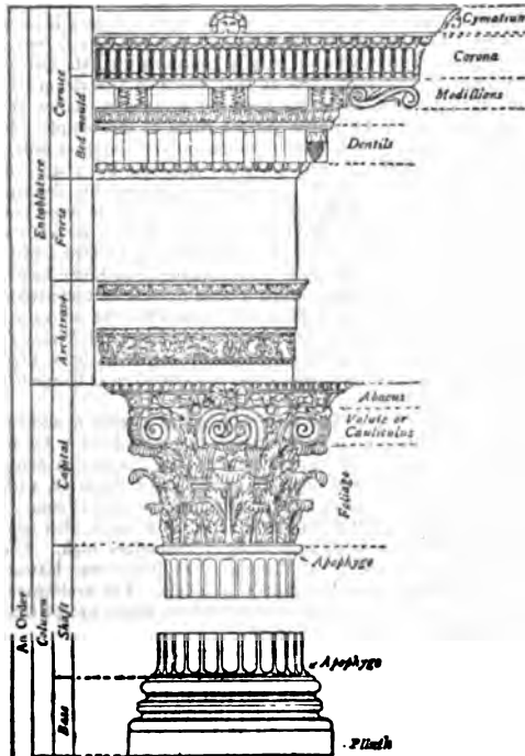
FIG. 11.—The Roman Corinthian Order: Temple of Castor.
