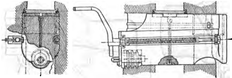
FIG. 32—Krupp Breech Action.
