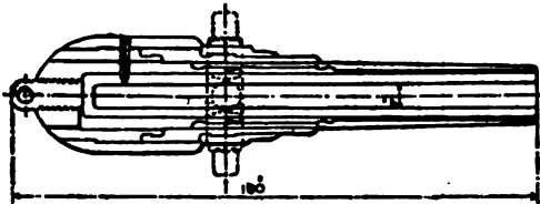
FIG. 12.—M.L. Gun Construction.
