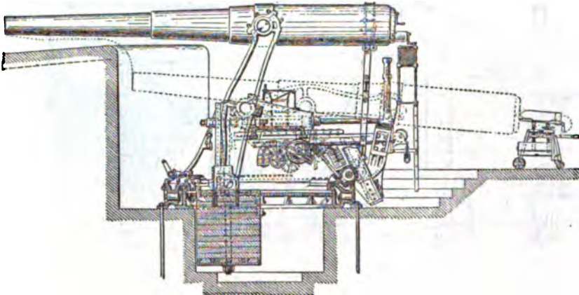
FIG. 81.—Buffington-Crozier Disappearing Carriage for 10° B.L. Gun, U.S.A.
