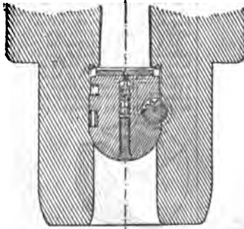
FIG. 33.—Krupp Breech Action.
