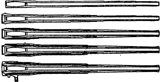
FIG. 14.—Modern B.L. Construction.
