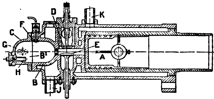
FIG. 14.—Crossley Oil Engine.
