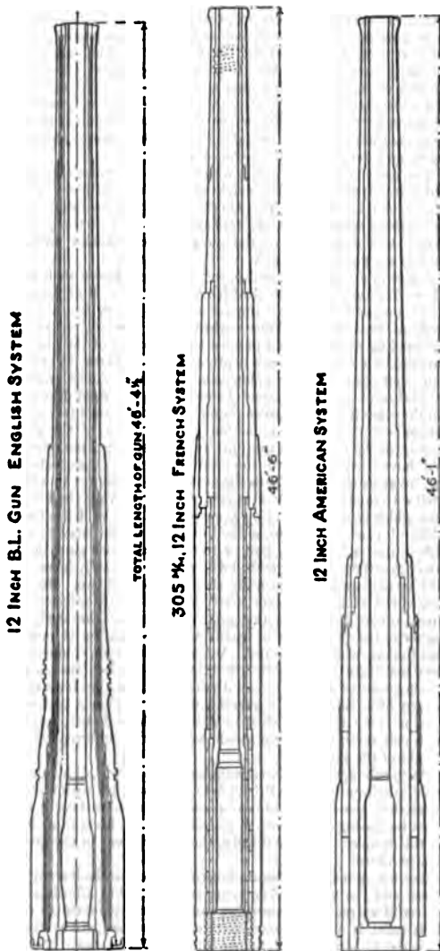
Figs. 55-57.—British, French and American Construction.
