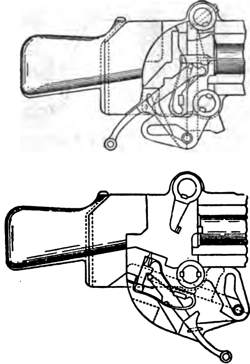
FIG. 35.—Nordenfeldt Q.F. Breech Mechanism.
