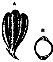
(After Renault.) FIG. 16.— Zygopteris pinnata . A, Group of sporangia, in surface view.
