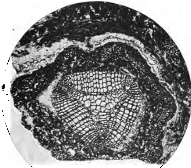
Fig. 4.— Palaeostachya pedunculata . Fertile shoot, bearing numerous cones and a few leaves. After Williamson (Scott, "Studies").
