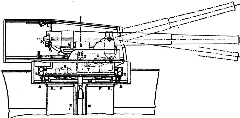
FIG. 92.—Diagram of a 9.2-in. Gun and Mounting, "Hogue" type.
