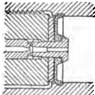
FIG. 48.—Elswick Cup.
