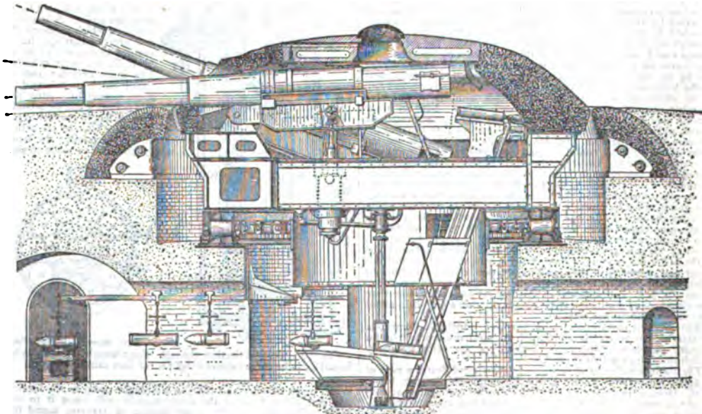
FIG. 82.—Krupp Cupola for two 28-cm. Guns.
