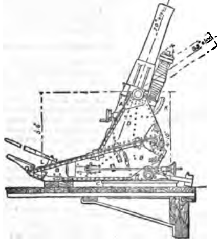
FIG. 73.—Diagram of British 6-in. B.L. Howitzer (70° elevation).
