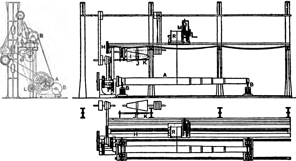
FIG. 20.—Wire-winding Machine.
