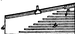
FIG. 8.—Wilfley Table.
