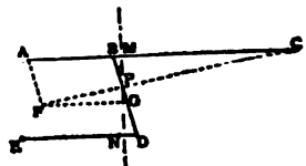
Watt's Parallel Motion.
