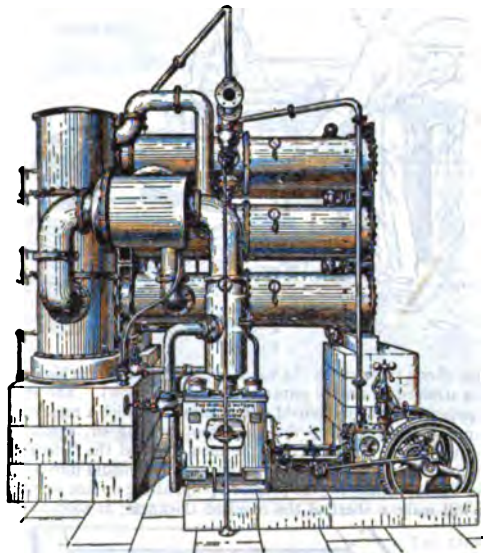
The Mirless Watson Co., Ltd. FIG. 7.—The Yaryan Patent Multiple Effect Evaporator.
