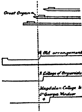
FIG. 14.—Relative Position of Manual and Pedal.
