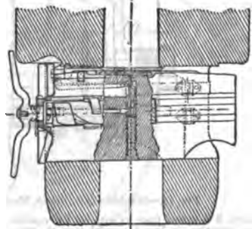
FIG. 33.—Krupp Breech Action.
