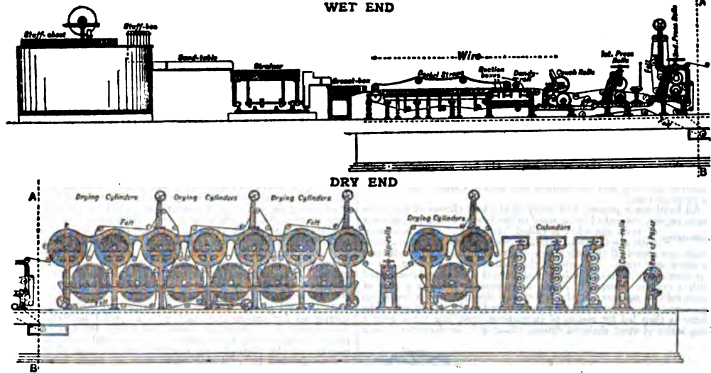
FIG. 12.—Paper-Making Machine.
