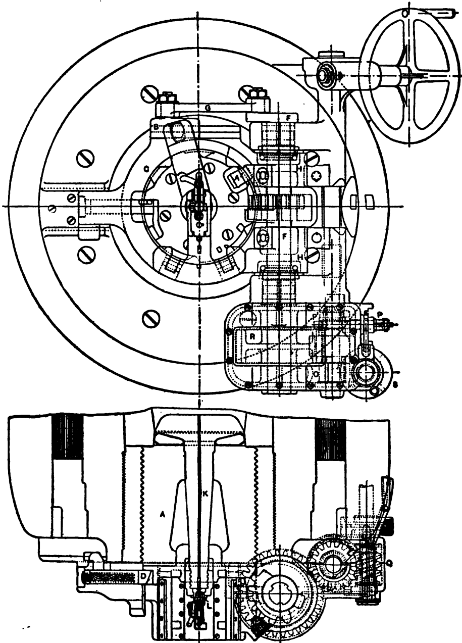
FIG. 41.—12-in. Gun, Breech Mechanism.
