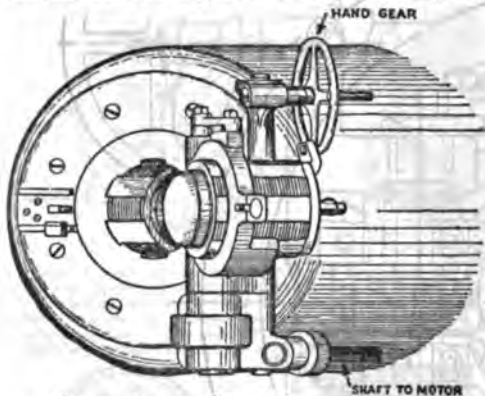
FIG. 37.—Interrupted Breech Screw—Cylindrical.
