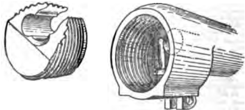
FIG. 36.—Eccentric Screw Breech Mechanism.
