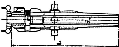
FIG. 11.—Armstrong B.L. Construction.
