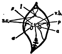
(After Stan. Scott, Studies.) FIG. 8.—Leaf-base of a Lepidodendron .
