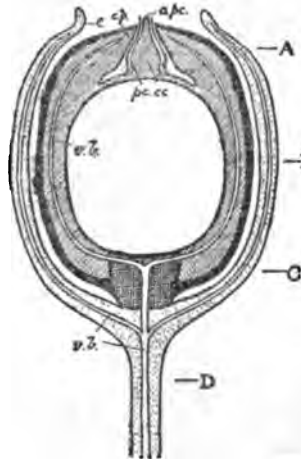
FIG. 26.— Lagenostoma Lomaxii . Diagram of seed in median longitudinal section.
