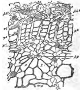
FIG. 21.— Heterangium Grievii . Part of the stele of the stem in transverse section, showing a primary xylem-strand and adjacent tissues. (X 135.)
