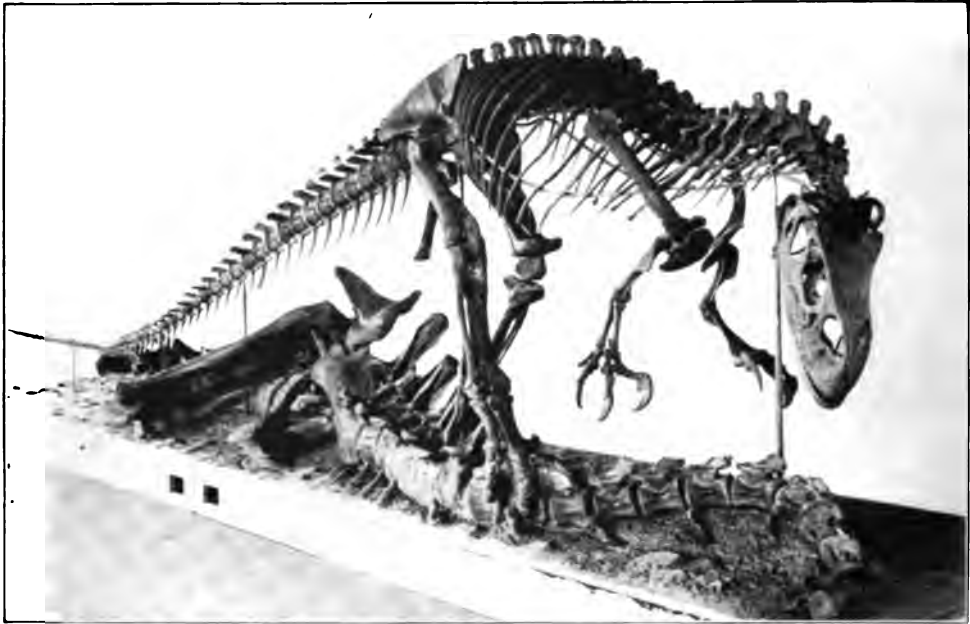
Fig. 4.—Skeleton of Allosaurus.
