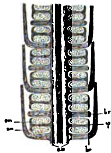
FIG. 2.— Calamostachys . Diagrammatic longitudinal section of the cone, showing the axis (ax) bearing alternate whorls of bracts (br) and peltate sporangiophores (sp) with their sporigonia (sm). The upturned tips of the bracts are only shown in every alternate verticil.
