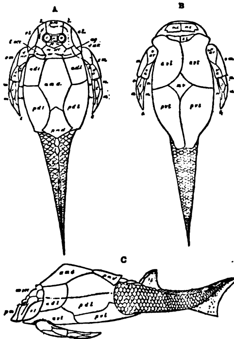
FIG. 4.— Pterichthys milleri , from the Middle Old Red Sandstone of Scotland, restored by Dr R. H. Traquair; upper (A), lower (B), and left-side view (C), about one-half nat. size.
