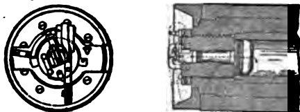
FIG. 42.—Breech Mechanism, 6-in. B.L. Mark IV.
